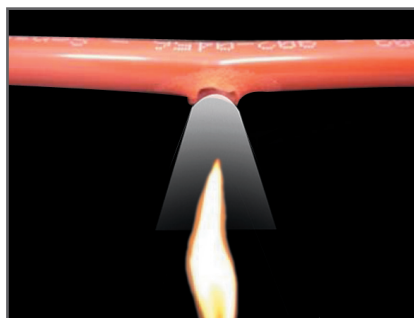
10 SECONDS tubing ruptures, releasing gas, extinguishing fire
