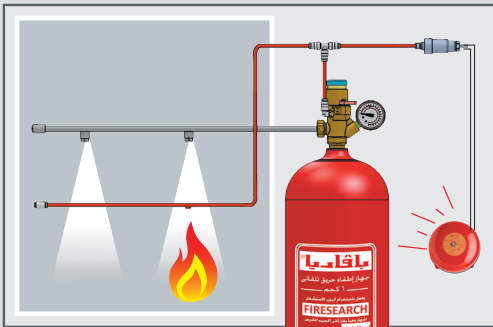
Indirect Pressure Operated System
